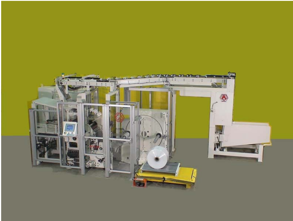
Photo showing 'fully-loaded' AFR-18 with options including special guard package, turret unwind and auto-core loading
