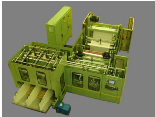
ELSNER MODEL RRW-1400 FULLY AUTOMATIC REWINDER
